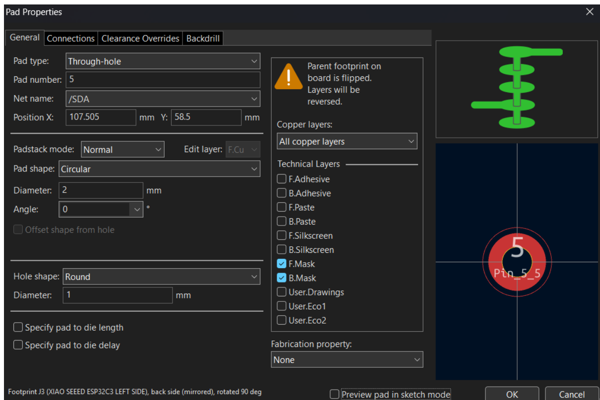
Figure 3.2: Pad Properties With Pad Review In Kicad PCB Editor
