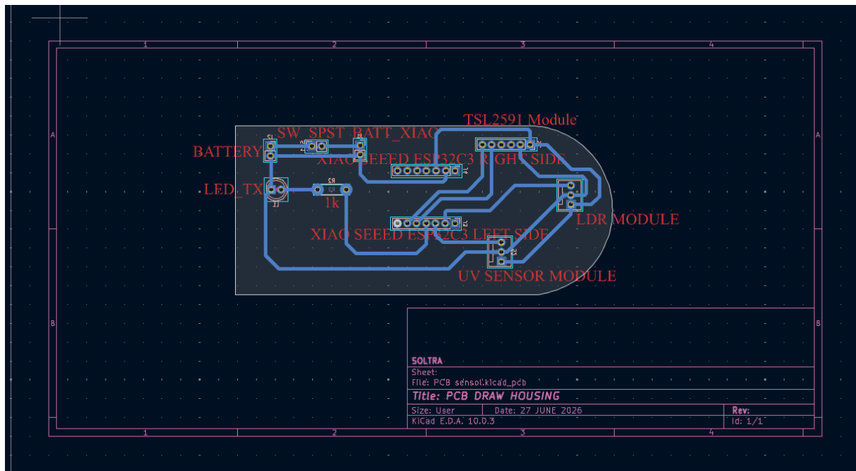
Figure 3.3: Full Pcb Connection In Kicad Pcb Editor
