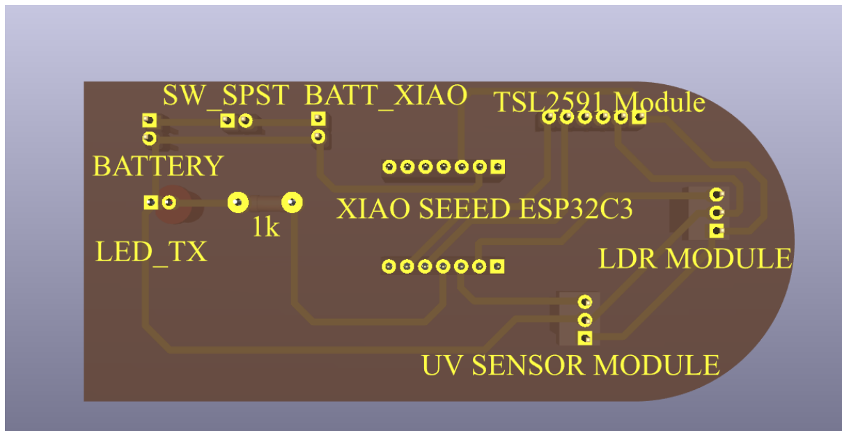
Figure 3.4: PCB In 3d Bottom View in Kicad PCB Editor
