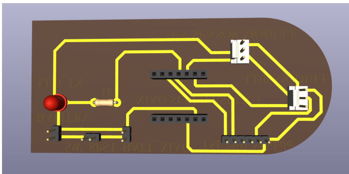
Figure 3.5: PCB In 3d Top View In Kicad PCB Editor
